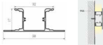
TR 10X12 GLASS PROFILE
