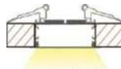
TR 150X35 CONCEAL
