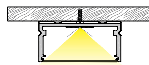
TR 50X12 CONCEAL
