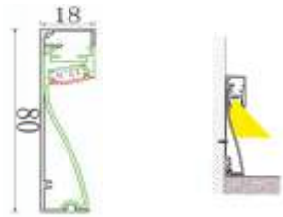
UP -DOWN PROFILE
