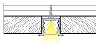
TR 17X7 BLACK +WH (CONCEAL)
