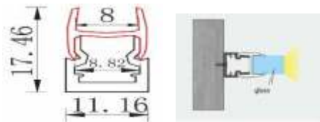
TR 10X12 GLASS PROFILE
