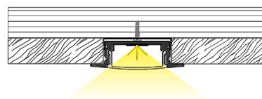
TR 11X7 CONCEAL
