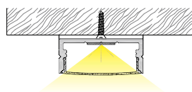
TR 25X9 SURFACE
