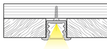
TR 10X10 CONCEAL
