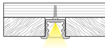
TR 7X9 CONCEAL
